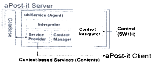
Fig. 3 The Architecture of aPost-it server
